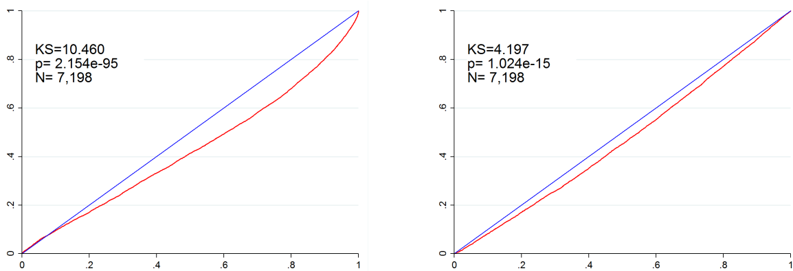
(a) First Serve: Empirical c.d.f. of t -values (b) Second Serve: Empirical c.d.f. of t -values
